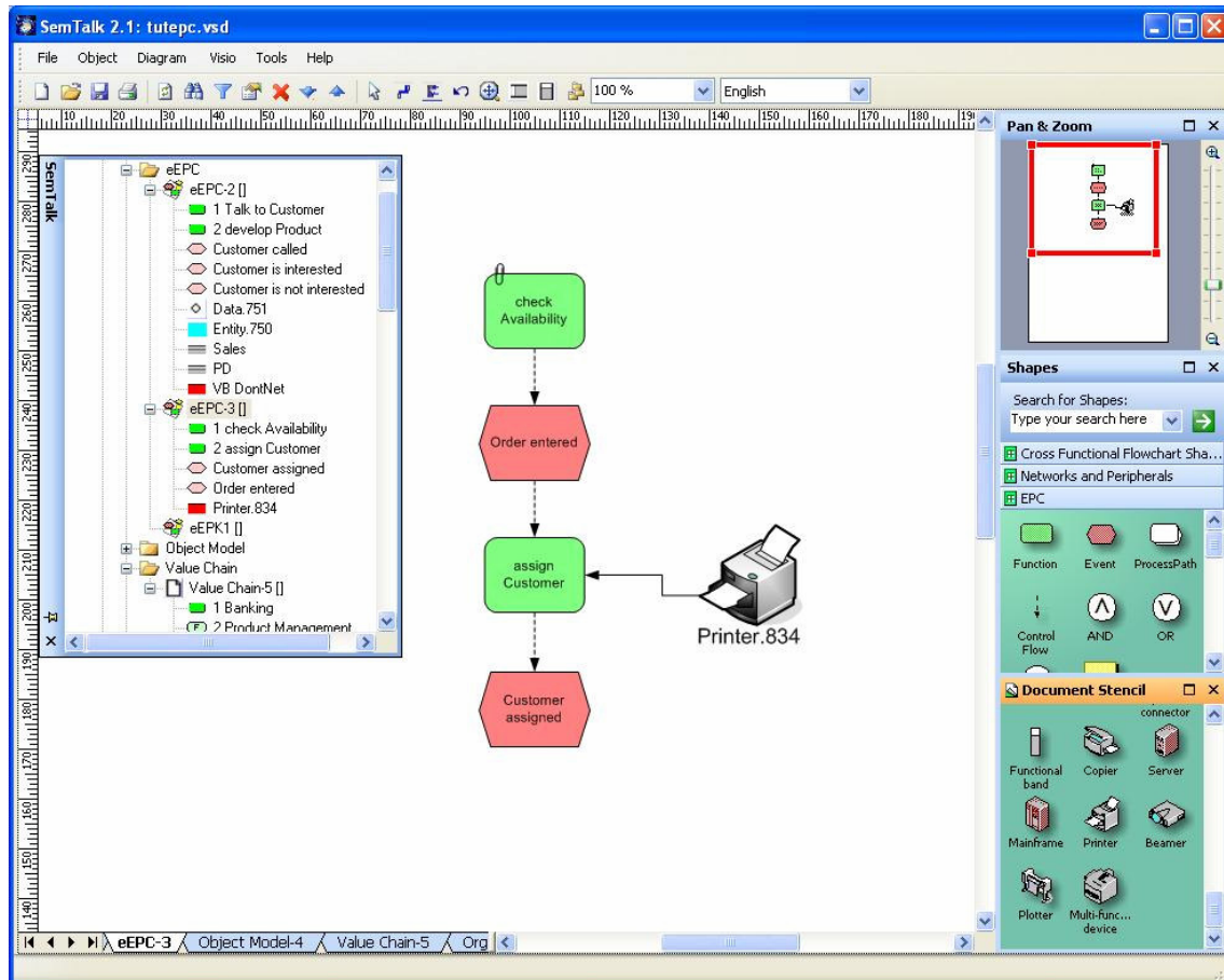
Figure 28: A Resource with a Visio Shape in a Process
