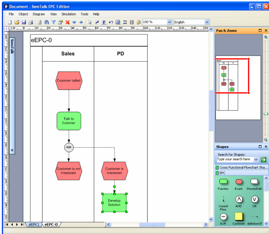
Figure 6: EPC with Swimlanes
