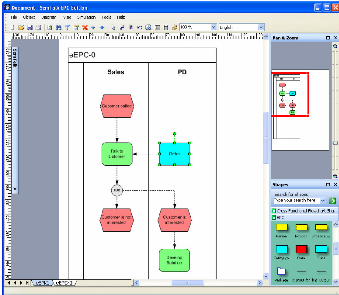
Figure 7: EPC with swim lanes and input / output
