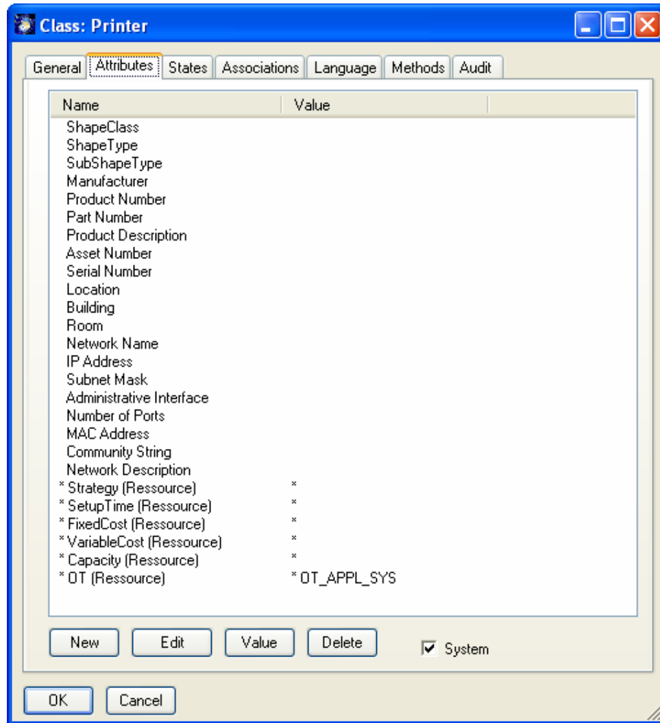
Figure 27: Attributes imported from Visio Masters
